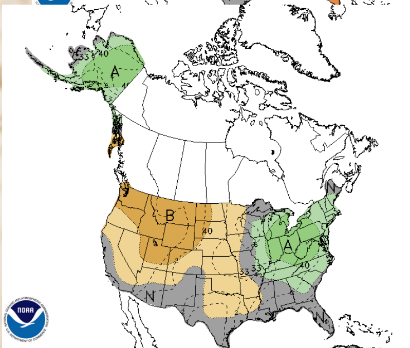
8-14 DAY OUTLOOK PRECIPITATION PROBABILITY MADE 3 AUG 2021 VALID AUG 11 - 17, 2021 DASHED BLACK LINES ARE CLIMATOLOGY (10THS OF INCHES). SHADED AREAS ARE FCS VALUES ABOVE (A) OR BELOW (B) NORMAL. GRAY AREAS ARE 'NEAR-NORMAL'
