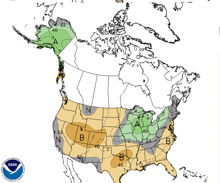
8-10 DAY OUTLOOK PRECIPITATION PROBABILITY MADE 3 AUG 2021 VALID AUG 09 - 13, 2021 DASHED BLACK LINES ARE CLIMATOLOGY (10THS OF INCHES). SHADED AREAS ARE FCS VALUES ABOVE (A) OR BELOW (B) NORMAL. GRAY AREAS ARE 'NEAR-NORMAL'
